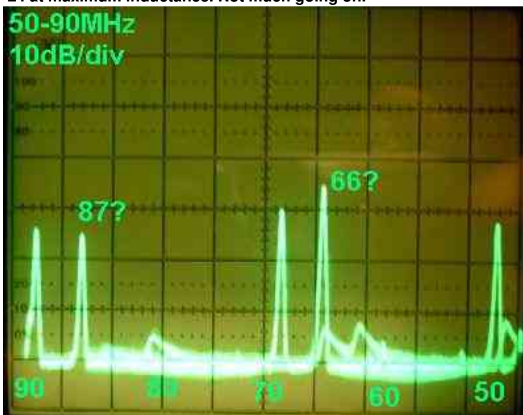
Decreasing the inductance of L4, signals suddenly snap in at about 66 and 86MHz (86MHz might
